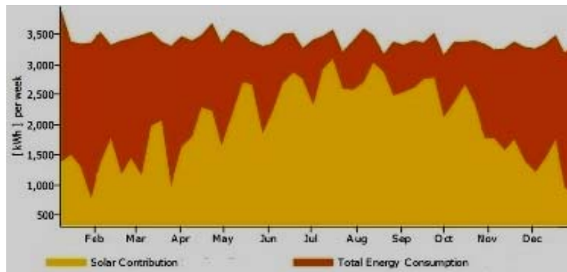
Fig. 1 Total energy required and energy produced by the solar system
