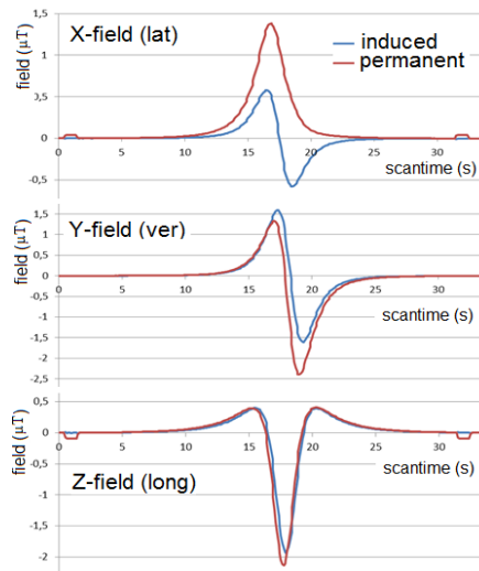
Fig. 3 Separation of permanent and induced signature. The horizontal axis shows time into the scan. Vertical axes show the field in all three directions
