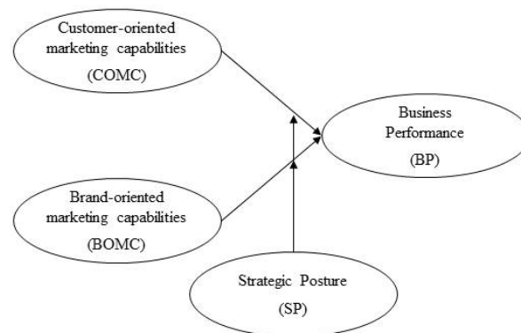
Fig. 1 Causal Model
