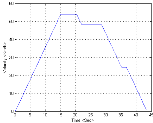
Fig. 6 Simplified Trajectory
