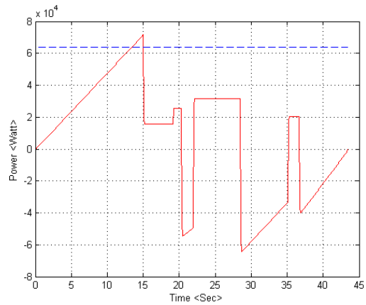
Fig. 8 TIBA 2 power for the respective trajectory
