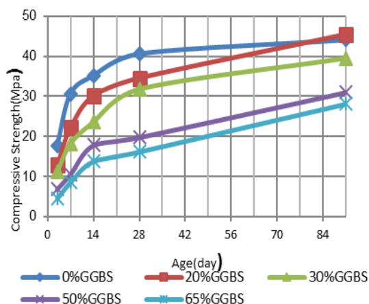
Fig. 11 Compressive strength development of NC by ages
