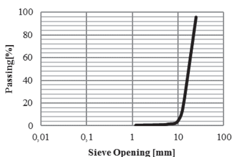
Fig. 2 Gravel grading
