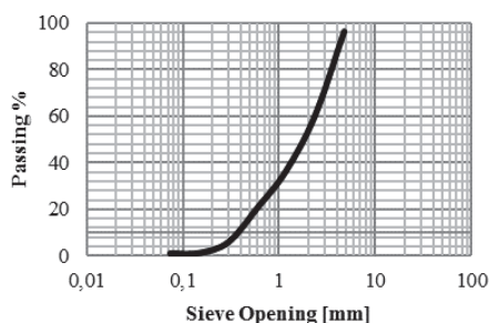
Fig. 1 Sand grading
