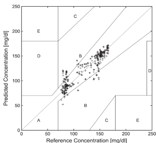
Fig. 3 Clarke Error Grid Analysis
