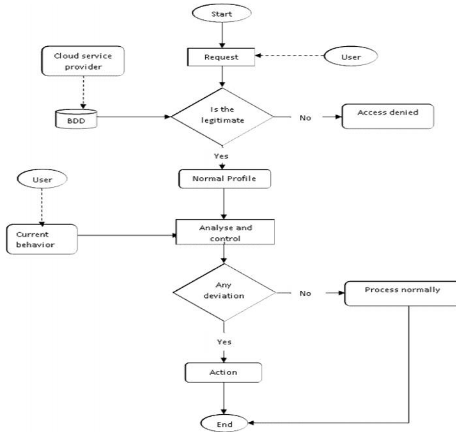
Fig. 2 IDS-activity framework
