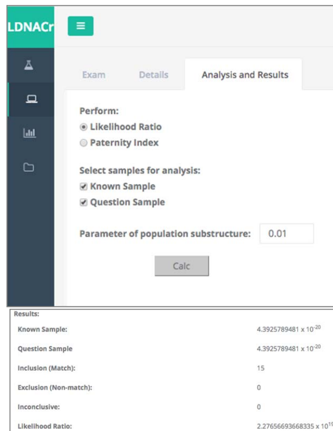
Fig. 3 Screenshots of section “Analysis and Results” showing a LR calculation and results
