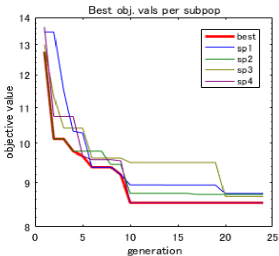
Fig. 3 Best objective values per subpopulation
