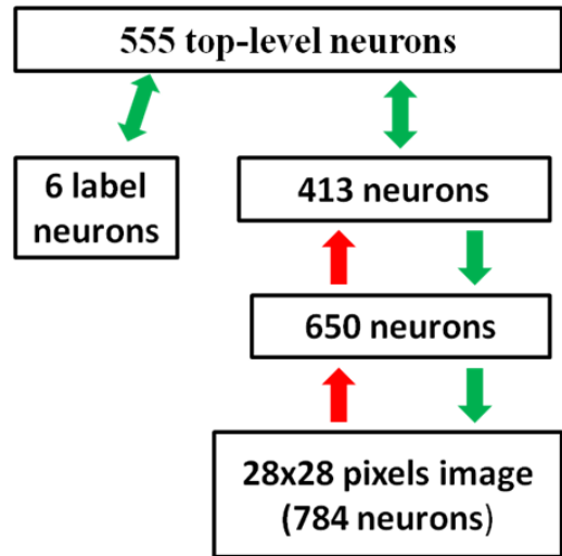
Fig. 2 Structure of our DBNN
