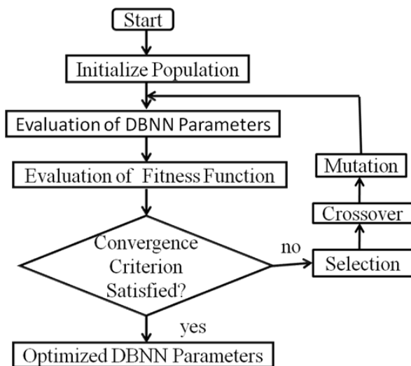
Fig. 1 Flowchart of combined GA and DBNN
