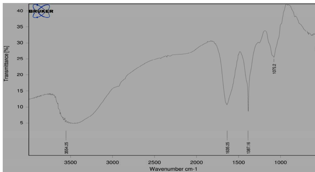
Fig. 5 FTIR spectrum of BSSNP
