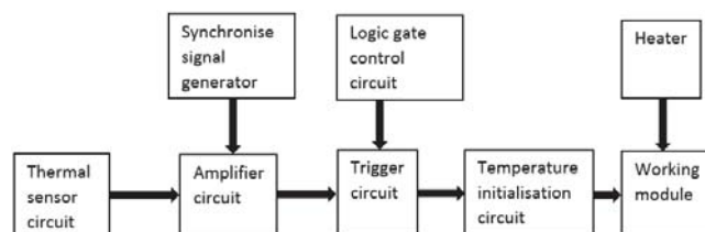
Fig. 1 System structure
