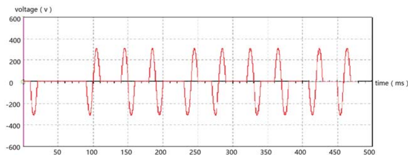
Fig. 10 Output voltage wave (e)
