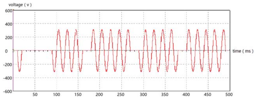
Fig. 7 Output voltage wave (b)
