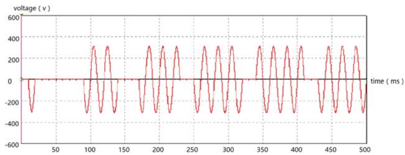
Fig. 8 Output voltage wave (c)
