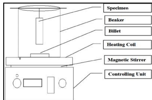
Fig. 3 Coating setup
