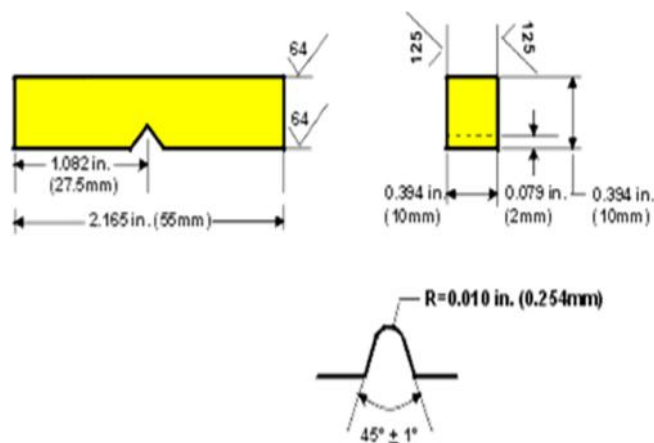
Fig. 5 Impact Test Specimen Specification
