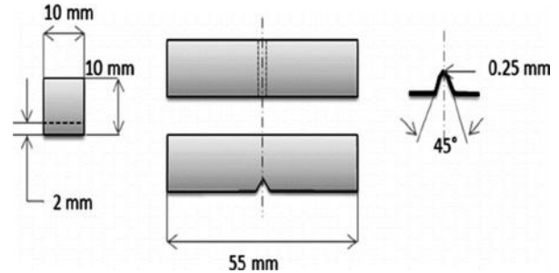
Fig. 1 Impact Specimen
