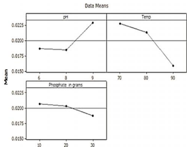
Fig. 10 Main effects plot for impact energy
