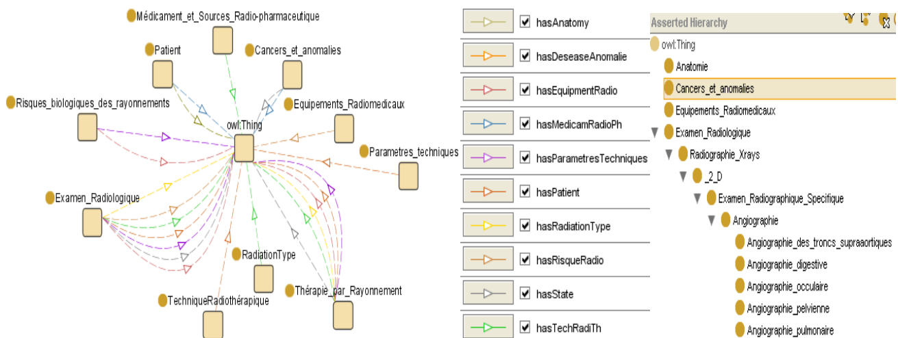
Fig. 2 Diagram of relationships between classes by « Jambalaya »
