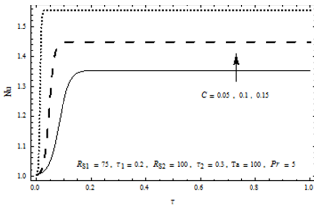
Fig. 5 Nusselt number Nu versus time \tau for different values of C
