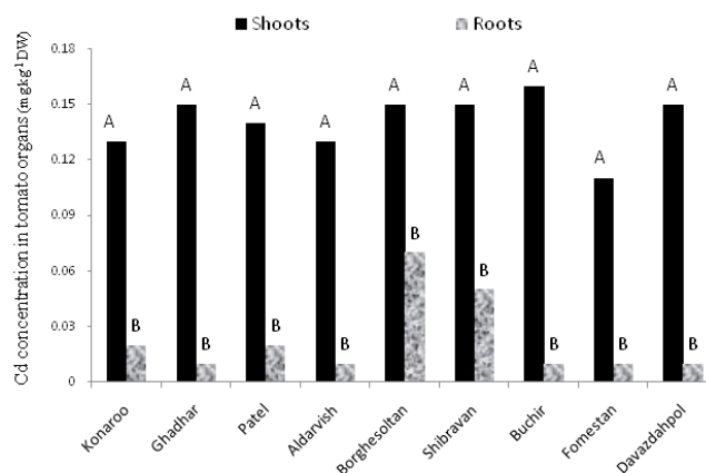
Fig. 1 Cadmium distribution in different tomato organs
