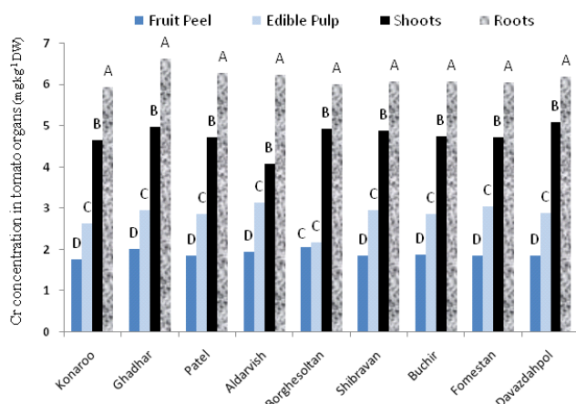
Fig. 2 Chromium distribution in different tomato organs
