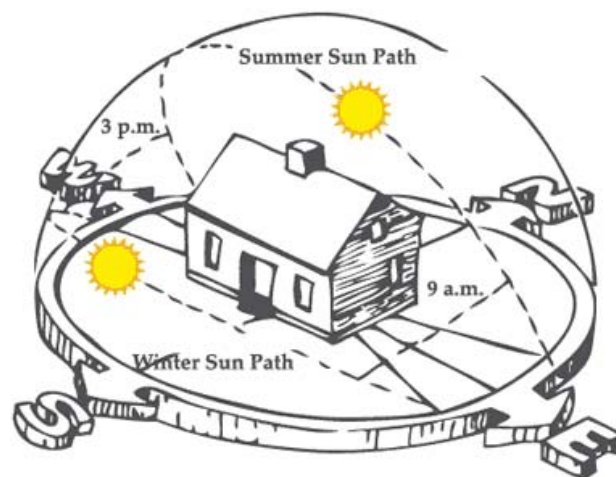
Fig. 1 Varying Sun-Path
