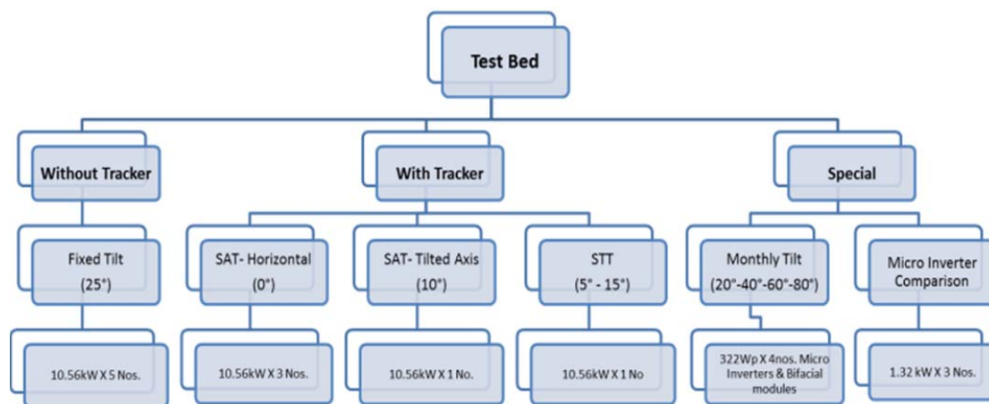
Fig. 4 Test Bed Plant Scheme
