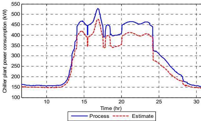
Fig. 4 Real-time performance of static chiller plant model
