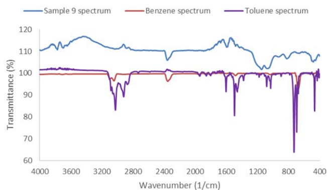
Fig. 12 Sample 9 spectrum
