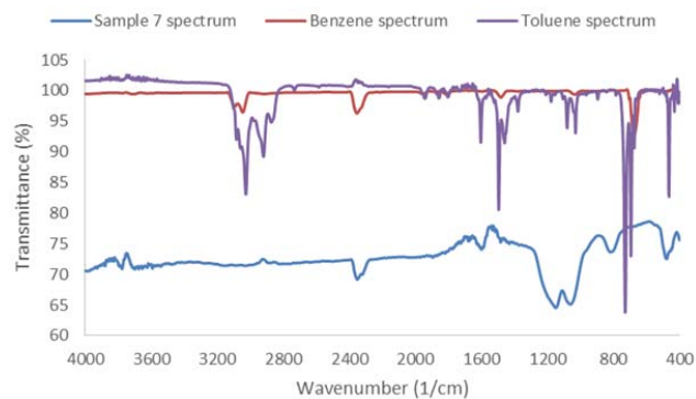
Fig. 11 Sample 7 spectrum
