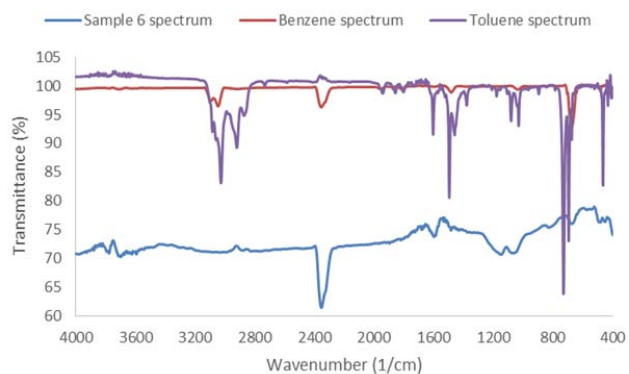
Fig. 10 Sample 6 spectrum
