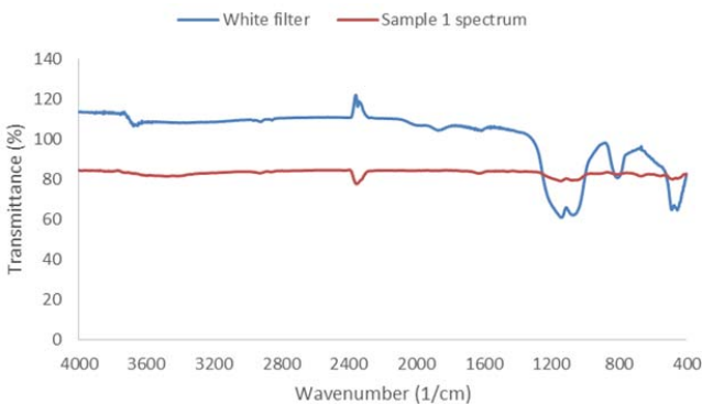
Fig. 5 White filter and Sample 1 spectrum
