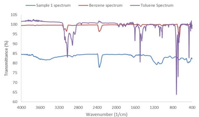
Fig. 6 Sample 1 spectrum
