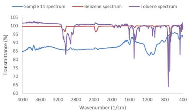
Fig. 13 Sample 11 spectrum
