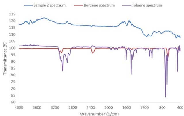
Fig. 7 Sample 2 spectrum
