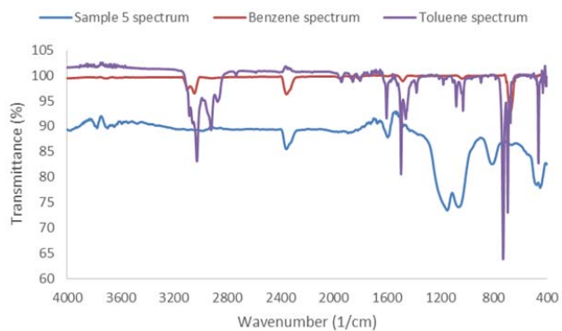
Fig. 9 Sample 5 spectrum
