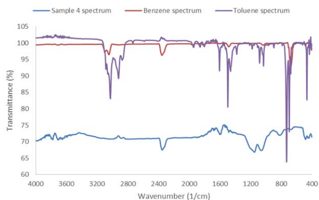
Fig. 8 Sample 4 spectrum
