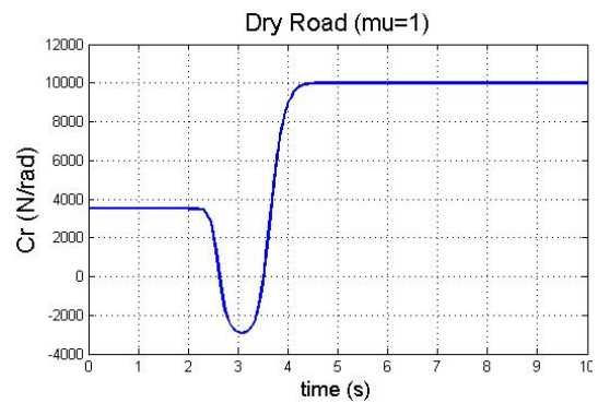
Fig. 5 Estimated rear cornering stiffness (dry road)
