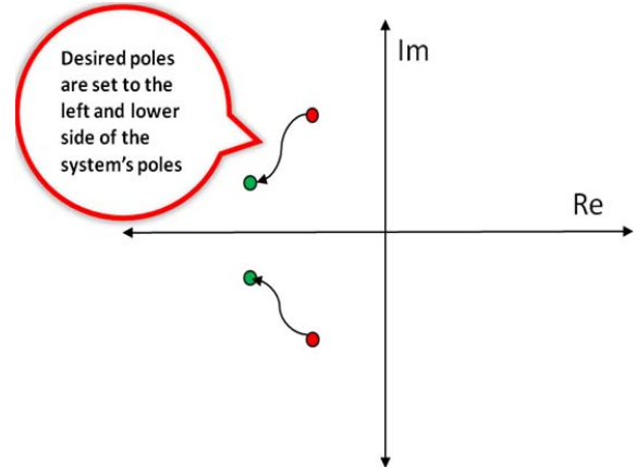
Fig. 2 Moving poles to the more stable zone
