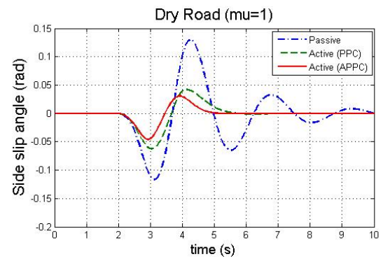
Fig. 6 Side slip angle (dry road)
