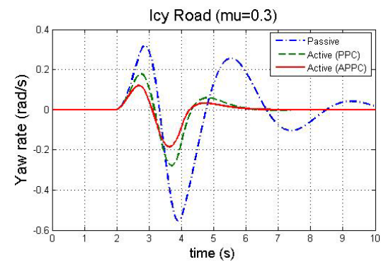
Fig. 15 Yaw rate (icy road)
