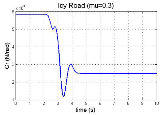
Fig. 13 Estimated rear cornering stiffness (icy road)
