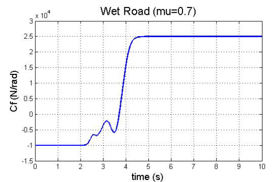
Fig. 8 Estimated front cornering stiffness (wet road)
