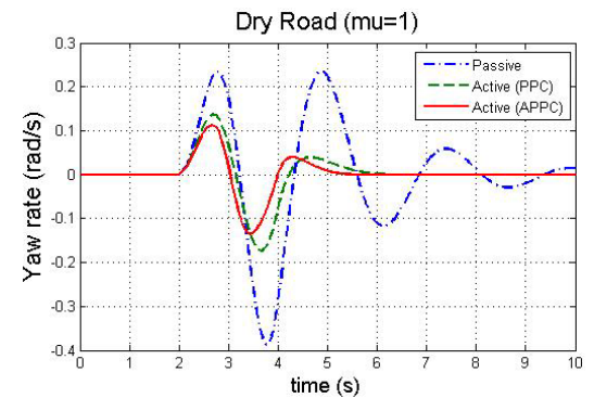
Fig. 7 Yaw rate (dry road)
