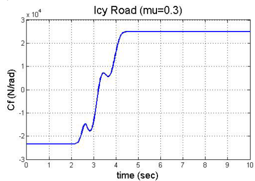
Fig. 12 Estimated front cornering stiffness (icy road)
