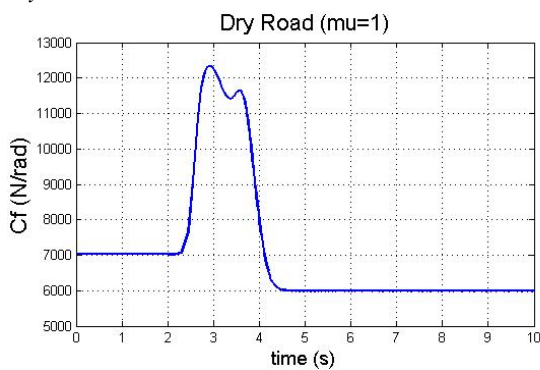
Fig. 4 Estimated front cornering stiffness (dry road)
