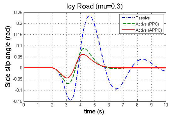
Fig. 14 Side slip angle (icy road)
