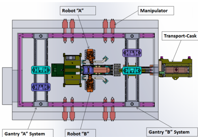
Fig. 3 ARC-Top View
