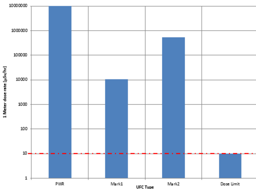
Fig. 2 Radiation dose rates (radial, gamma -1m)
