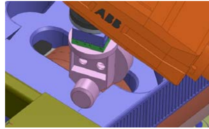
Fig. 8 UFC Grinding (or Milling)- using Robot “B”
