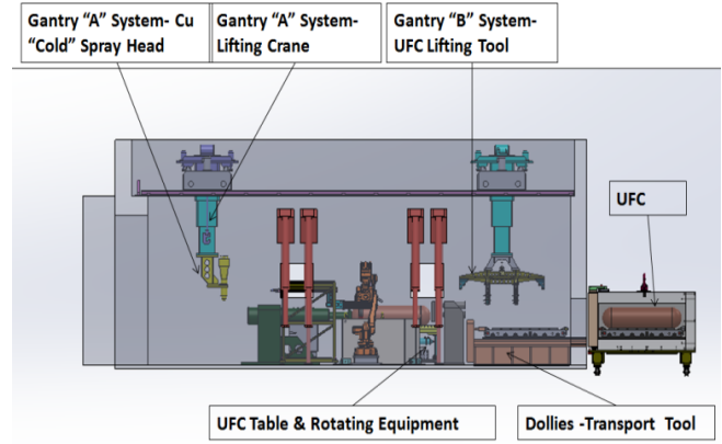
Fig. 4 ARC-Side View
