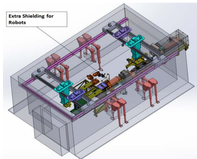
Fig. 5 ARC-ISO View
