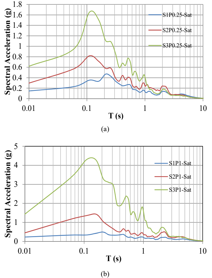
Fig. 8 Spectral acceleration (5% damping) calculated from acceleration time history recorded at the pile top in different soil types saturated conditions: (a) PGA = 0.25, (b) PGA = 1.
