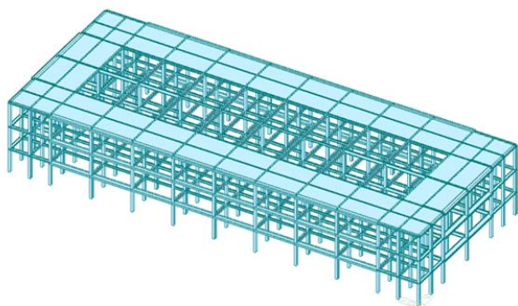
Fig. 4 Structural modeling of the example building
