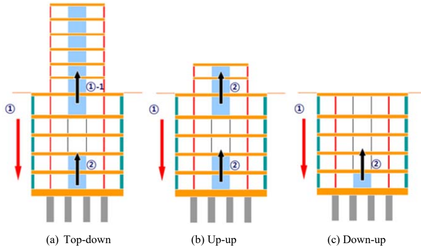
Fig. 1 Construction processes of Top-down method
