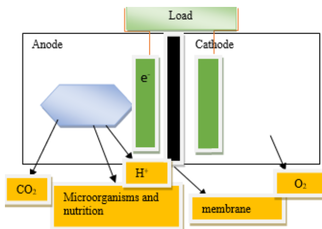
Fig. 2 General schematic of a microbial fuel cell
