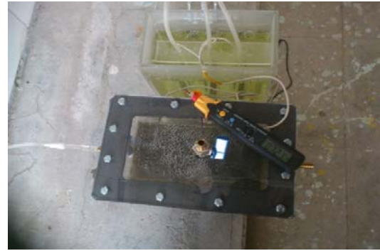
Fig. 3 The microbial fuel cell built for this research
