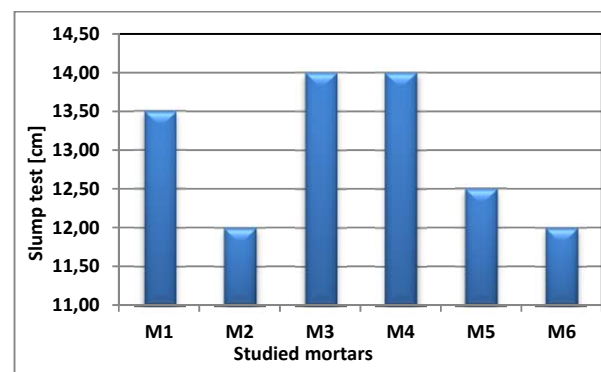
Fig. 2 Slump a function of nature of cement
