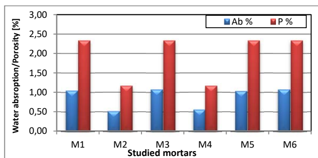
Fig. 4 Porosity a function of nature of cement
