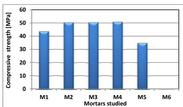
Fig. 6 Compressive strengths of different mortars
