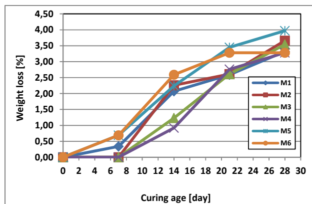
Fig. 7 Mass loss of the different mortars for a period of 28 days
