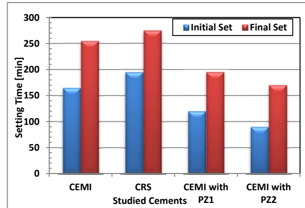
Fig. 1 Setting time a function of nature of cement
