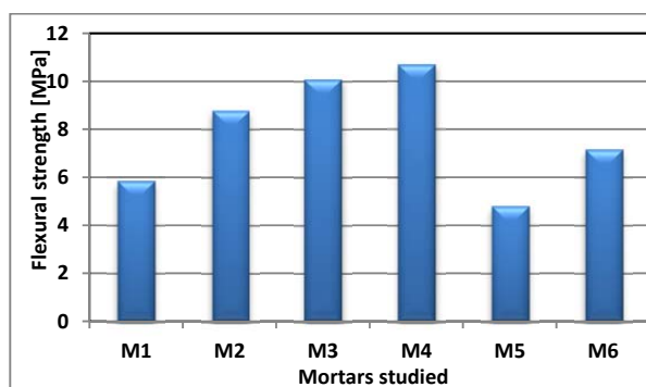
Fig. 5 Flexural strengths of different mortars
