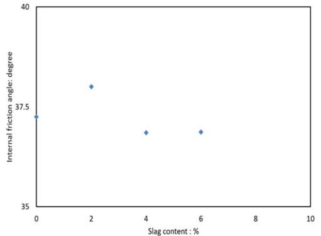
Fig. 7 Internal friction angle vs. slag content
