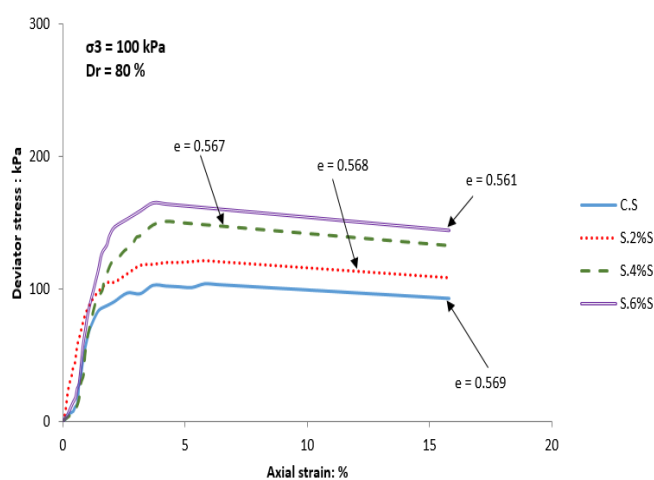
Fig. 9 Stress-strain curves for tests on sand-slag specimens
