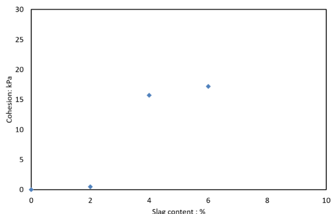
Fig. 8 Cohesion vs. slag content
