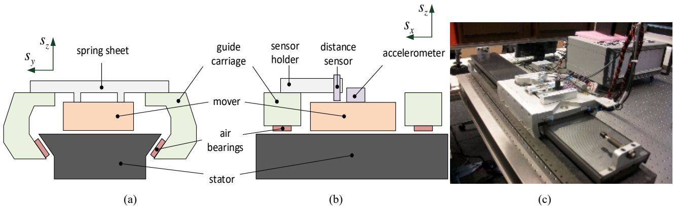
Fig. 2 Experimental setup; schematic cutaway of front (a) and side view (b) and test rig (c). The linear drive is located on a massive table with a breadboard
