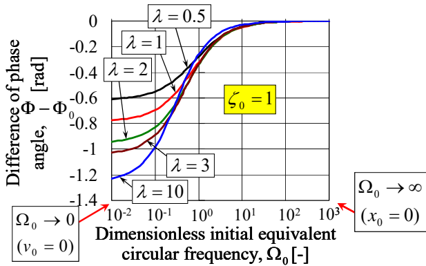
Fig. 17 Variation of the difference of phase angle versus the dimensionless initial equivalent circular frequency, for various values of the dimensionless inertia and \zeta_0 = 1
