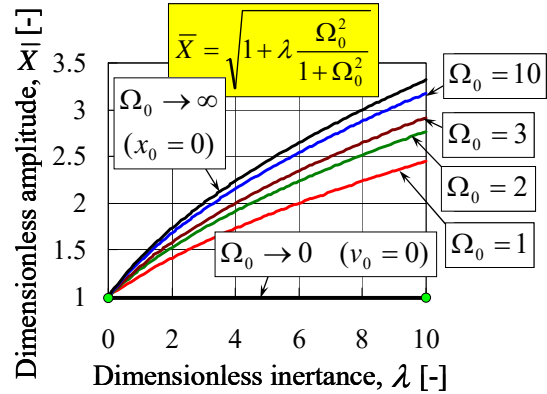
Fig. 4 Variation of the dimensionless amplitude versus the dimensionless inertance, for various values of the dimensionless initial equivalent circular frequency
