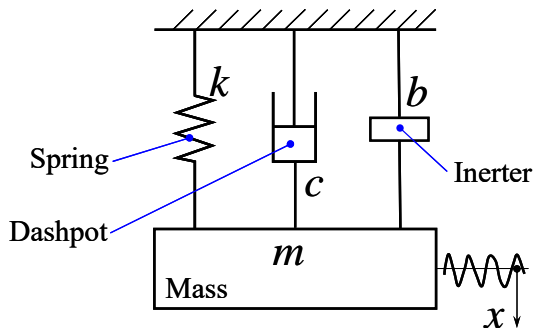
Fig. 2 Schematic view of the damped 1DOF vibration system, in which the mass element is suspended by an elastic element connected in parallel with a dissipative element and an inerter
