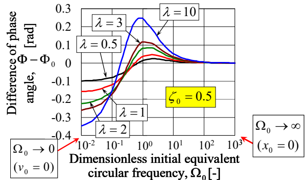
Fig. 15 Variation of the difference of phase angle versus the dimensionless initial equivalent circular frequency, for various values of the dimensionless inertance and \zeta_0 = 0.5
