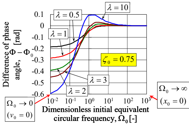
Fig. 16 Variation of the difference of phase angle versus the dimensionless initial equivalent circular frequency, for various values of the dimensionless inertia and \zeta_0 = 0.75
