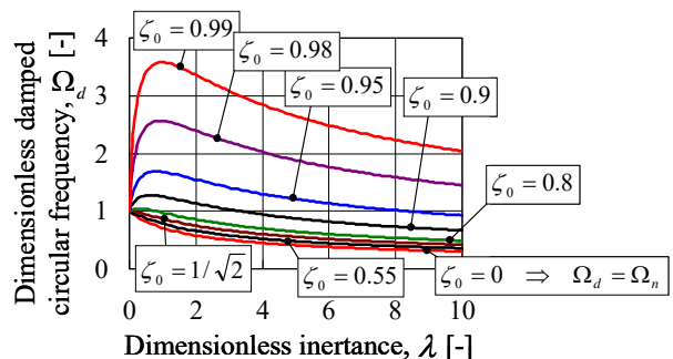
Fig. 10 Change of the dimensionless damped circular frequency versus the dimensionless inertia, for various values of the damping ratio
