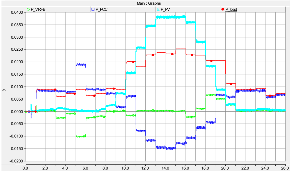
Fig. 12 Dynamic characteristics of scheduled operation
