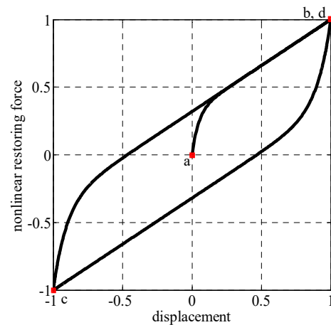
Fig. 1 Typical normalized symmetric softening force-displacement loop
