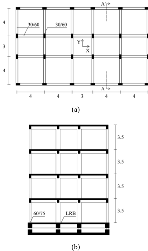
Fig. 3 Four-story reinforced concrete base-isolated structure: (a) typical floor plan; (b) section A-A'
