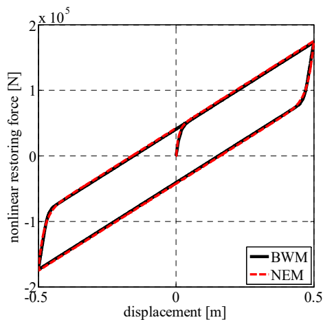
Fig. 4 Simulated force-displacement hysteresis loops
