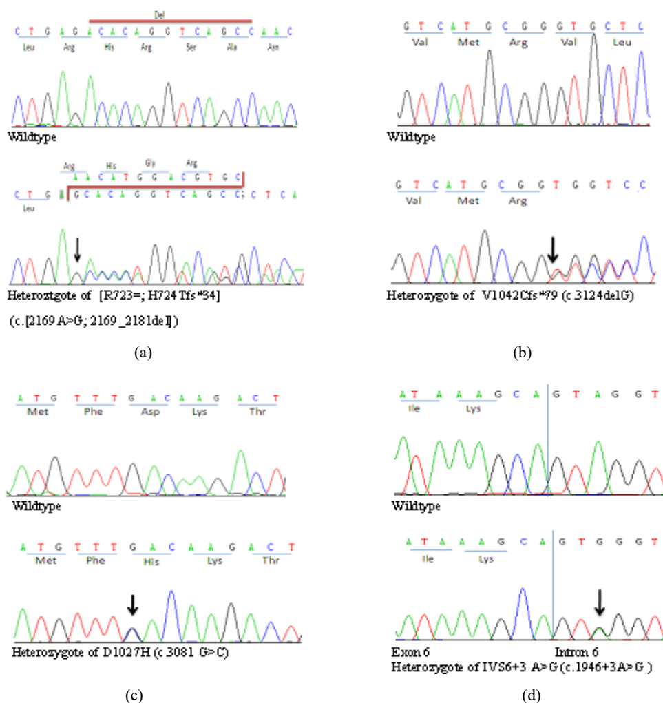
Fig. 2 Sequence analysis of the four novel mutations of the ATP7B gene. a . A 13-bp (ACACAGGTCAAGCC) deletion (accompanied by a changed base pair [A>G at nucleotide 2169, a polymorphism]) from nucleotide 2169_2181 (codon 724) of exon 8 in patient 1. The frame shift results in a truncated protein by introduced a new stop codon at position 758; b . A one-bp (G) deletion at nucleotide 3124 (codon 1042) of exon 14 from patient 2. The in-frame deletion results in introducing a new stop codon (codon 1121); c . D1027H (c.3081G>C) from patient 3; d . IVS6+3A>G (c.1946+3A>G) from patient 4
