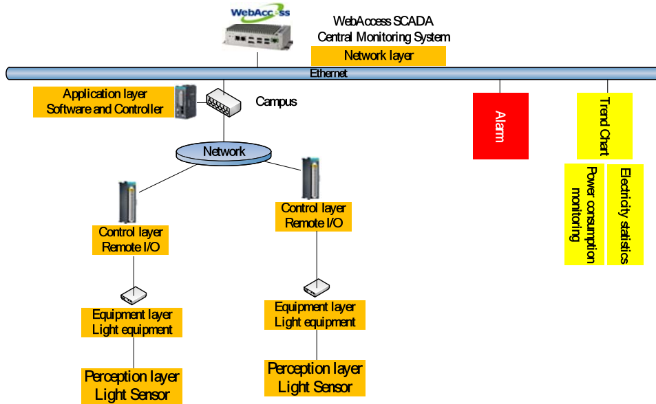
Fig. 2 The block diagram of proposed system
