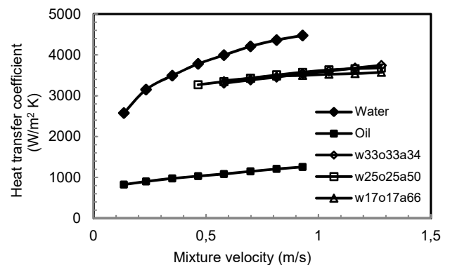
Fig. 7 Variation of heat transfer coefficients for water-oil-air three-phase flow with mixture velocity
