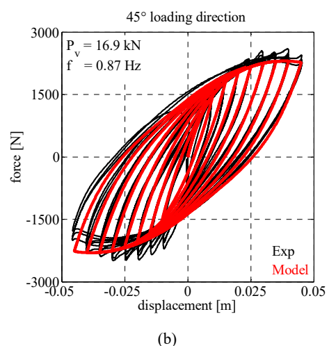
Fig. 13 Analytical and experimental hysteresis loops in: (a) 0^\circ and (b) 45^\circ loading directions
