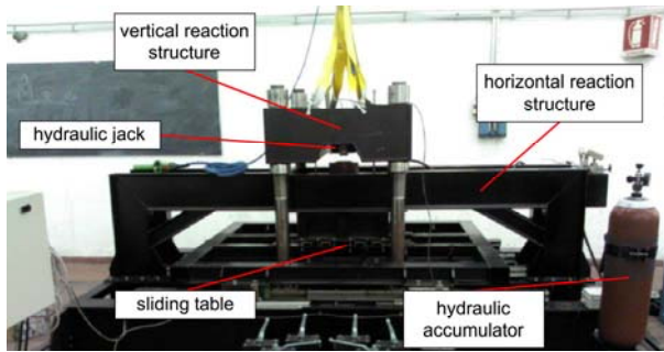
Fig. 6 Testing machine
