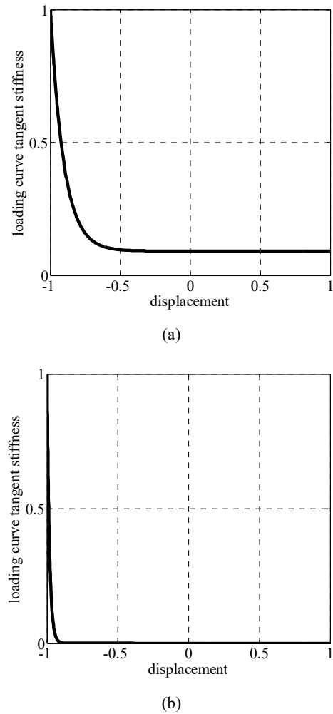
Fig. 2 Tangent stiffness variation of the loading curve with (a) bilinear and (b) rigid-plastic characteristics
