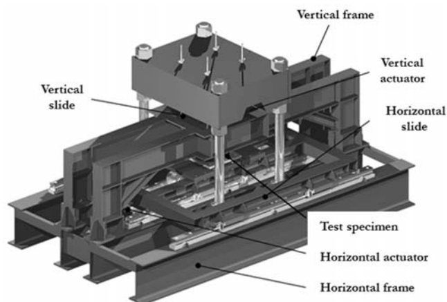
Fig. 2 Testing machine
