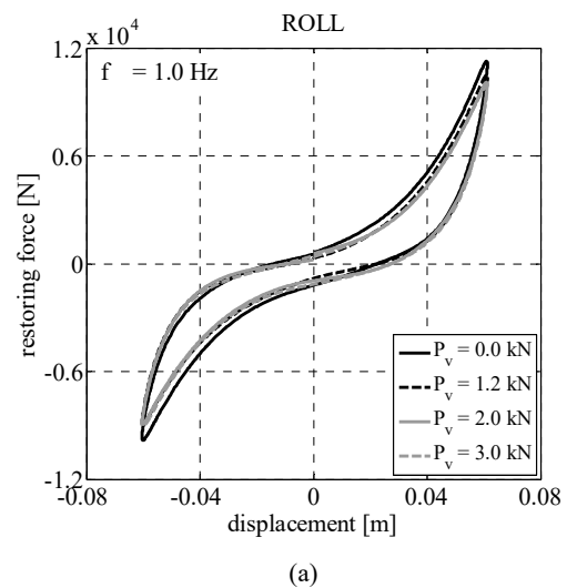
Fig. 8 Influence of vertical load at relatively large displacements in (a) Roll and (b) Shear directions
