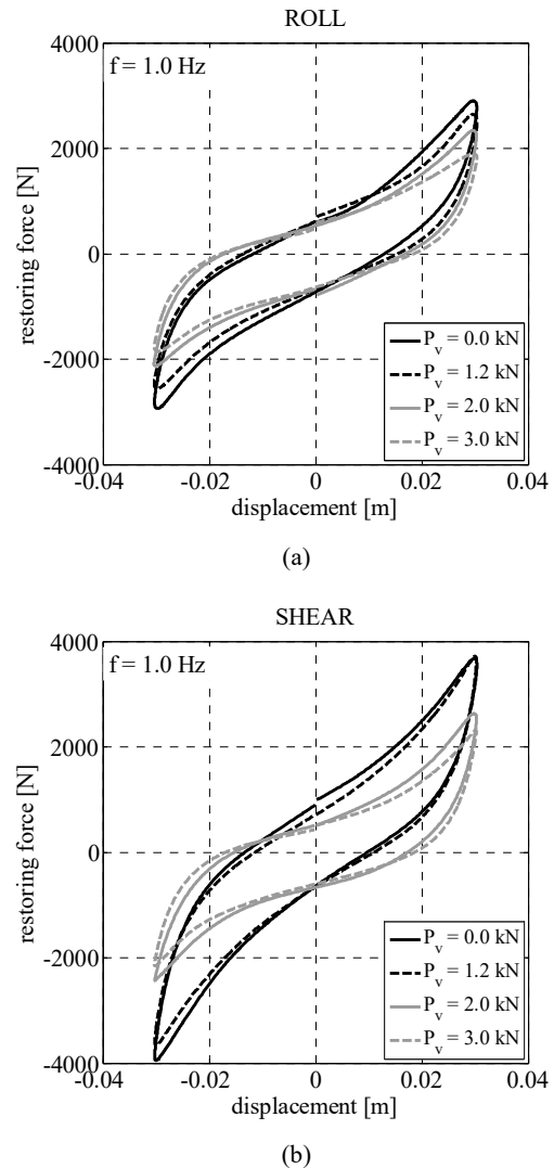
Fig. 8 Influence of vertical load at relatively large displacements in (a) Roll and (b) Shear directions
