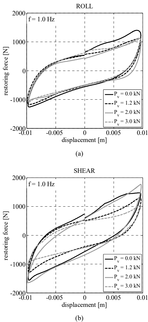
Fig. 7 Influence of vertical load at small displacements in (a) Roll and (b) Shear directions
