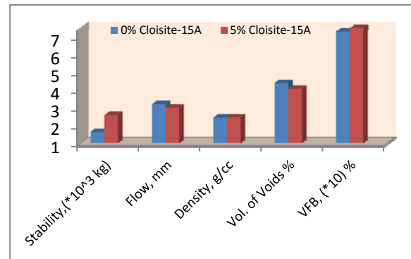
Fig. 10 Marshall Test results
