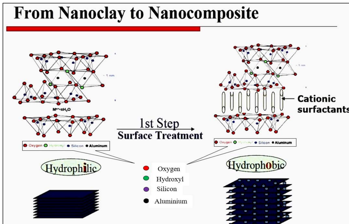
Fig. 1 Surface treatment of nanoclay
