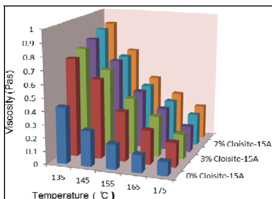
Fig. 6 Effect of Cloisite-15A on viscosity
