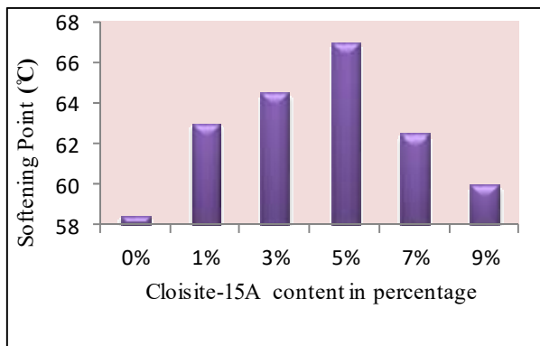
Fig. 5 Effect of Cloisite-15A on softening point
