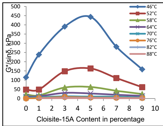
Fig. 9 Effect of Cloisite-15A on rutting resistance
