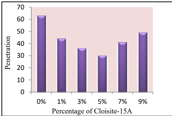
Fig. 4 Effect of Cloisite-15A on penetration
