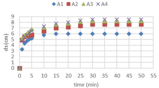
Fig. 3 Evolution in scour depth according to different time for sample (A)
