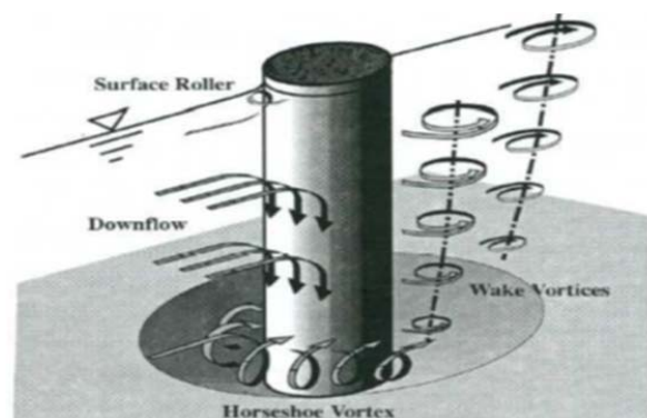
Fig. 1 Vortex motion around a pier [7]
