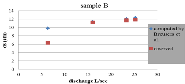
Fig. 7 Comparison between observed and computed of scour depth for sample B
