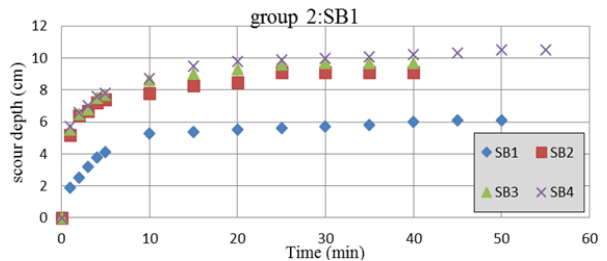
Fig. 4 Evolution in scour depth according to different time for sample (B)
