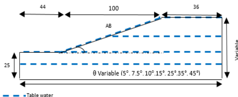
Fig. 3 Geometry of the reference model studied.
