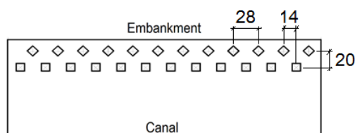
Fig. 4 Pattern of piles group
