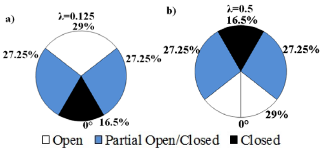
Fig. 8 Statuses of a crack in the balanced shaft during a shaft rotation at crack locations (a) \lambda = 0.125 and (b) \lambda = 0.5
