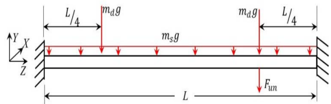
Fig. 1 A rigidly supported two-disk rotor
