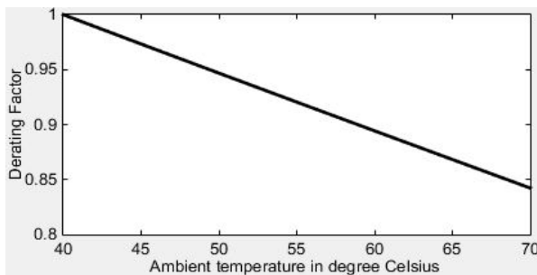
Fig. 7 De-rating factor versus ambient temperature
