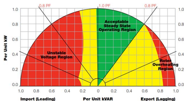
Fig. 1 Typical generator reactive capability curve [4]
