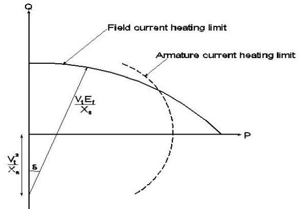
Fig. 4 Generator field current limit [8]
