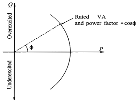
Fig. 2 Generator armature current limit [8]
