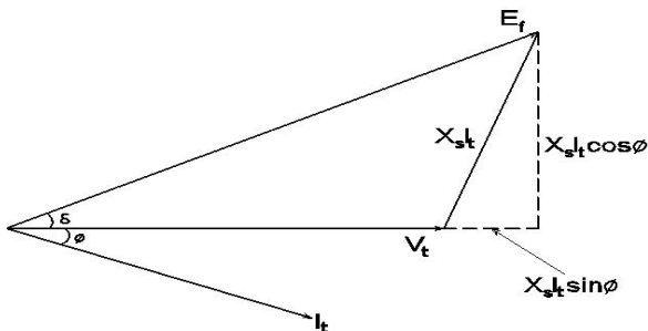
Fig. 3 Synchronous generator phasor diagram [8]
