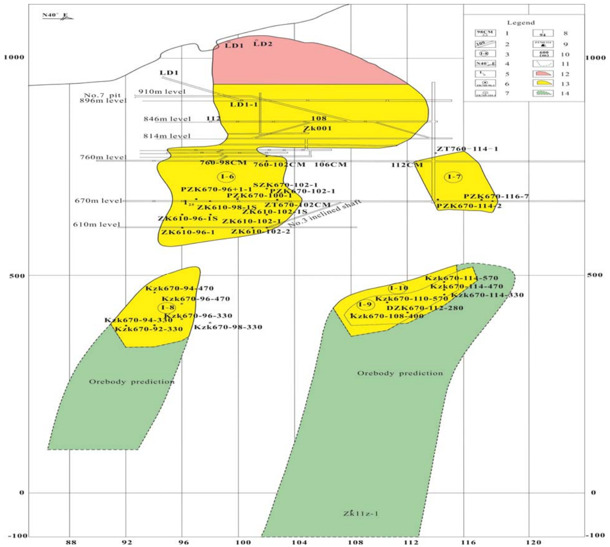
Fig. 3 Projection profile of concealed ore-bodies found newly at No. 1 mineralized belt in the Maoping Zn-Pb-(Ag-Ge) deposit 1. Transverse drift; 2. Inclined; 3. Ore-body number; 4. Azimuth; 5. Station; 6. Ore drilling; 7. Not ore drilling; 8. Exploration line; 9. Sampling number; 10. Elevation; 11. Boundary resources (above 333) grade; 12. Oxidized ore-bodies; 13. Sulfide ore-bodies; 14. Predicted ore-body positioning. Especially, it is suitable for accurate positioning for concealed ore-bodies on 1:500 ~ 1:10000 scales
