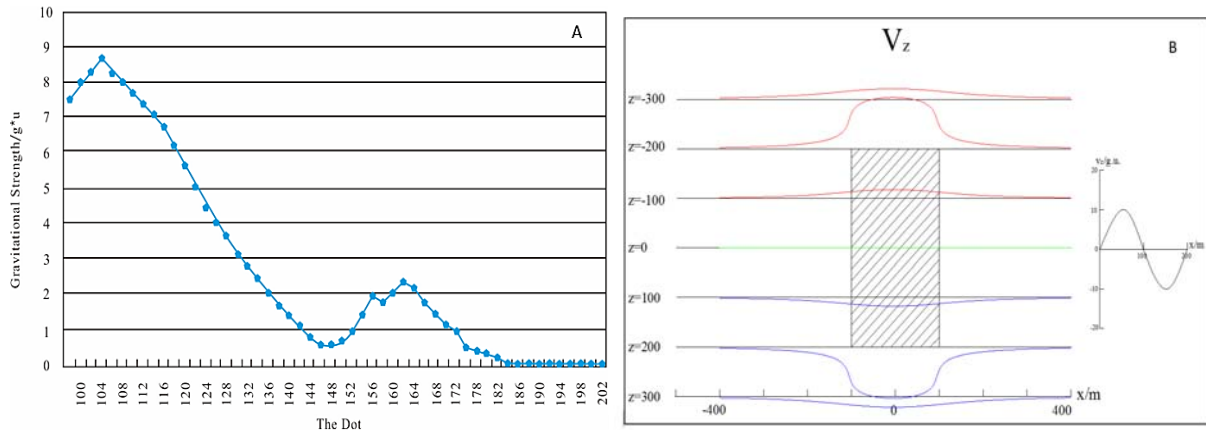
Fig. 2 The tunnel gravity measurement of three dimensional unusual Significance: A. The gravitational strength of the dot. B. The sketch of the tunnel gravity measurement of three dimensional unusual significance
