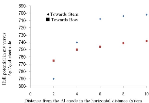
Fig. 7 Potential distribution in horizontal direction (X) towards bow and stern the ship model vs. Ag/Ag Cl ref. electrode by V
