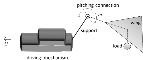
Fig. 1 Traction flight vehicle
