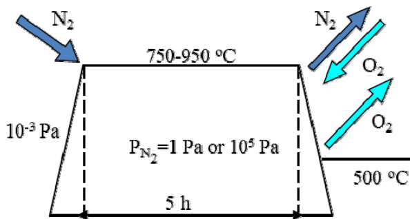
Fig. 2 Oxynitriding process of Ti-6Al-4V alloy
