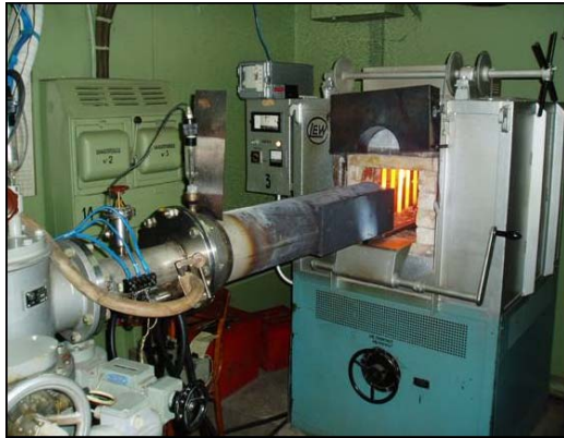
Fig. 1 Oxynitriding equipment
