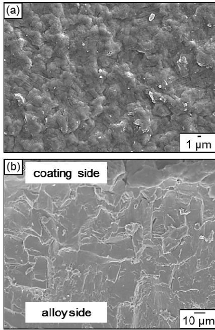
Fig. 4 SEM microstructures of the Ti-6Al-4V alloy after oxynitriding at 750 °C under P_{N_2}=10^5 Pa: (a) top view, (b) fracture surface
