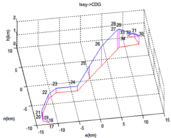
Fig. 7 3D mission profile from Issy to CDG
