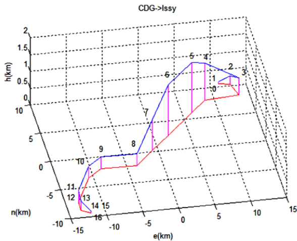
Fig. 6 3D mission profile from CDG to Issy
