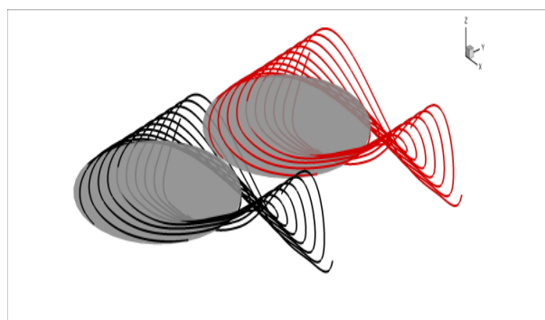
Fig. 17 Tip vortex geometry predicted by the noise module for the X015-5 tandem in approach
