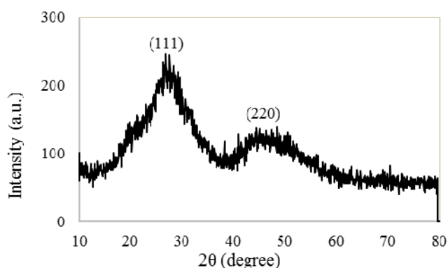
Fig. 2 The XRD pattern of biosynthesized CdS nanoparticles
