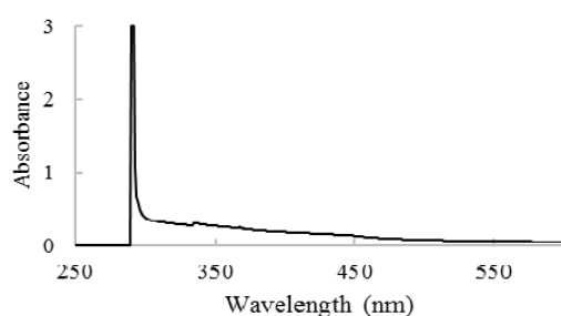
Fig. 6 UV-Vis spectra of biosynthesized CdS nanoparticles
