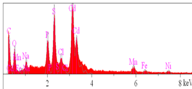
Fig. 3 EDS analysis on the nanoparticles produced from the Ni- Cd cake
