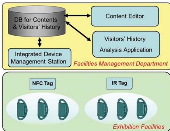
Fig. 1 The basic architecture of the guide system
