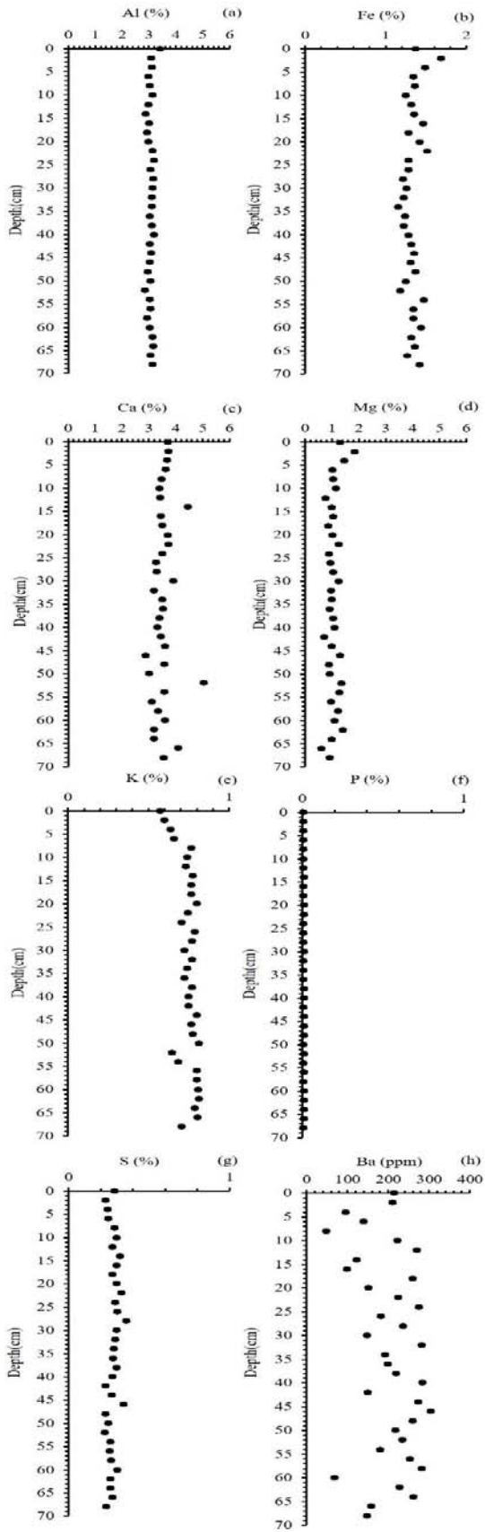
Fig. 2 (a)-(h) Down core variations of metals
