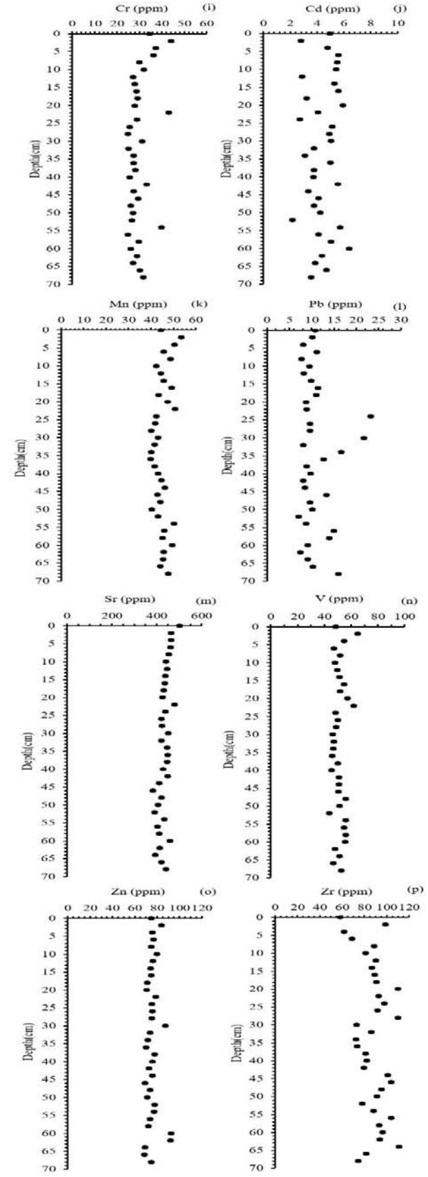
Fig. 2 (i)-(p) Down core variations of metals
