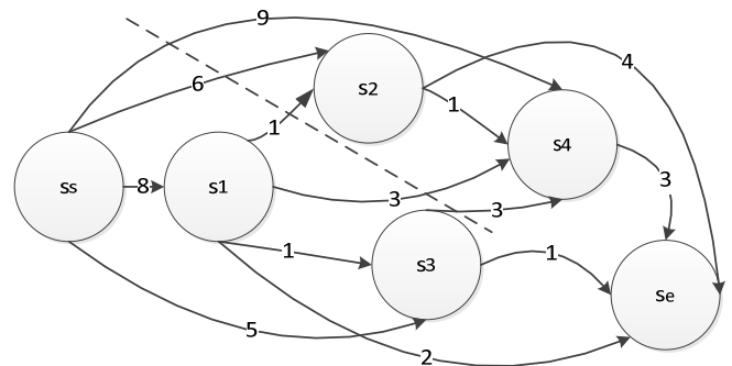
Fig. 4 Dinic algorithm segmentation results
