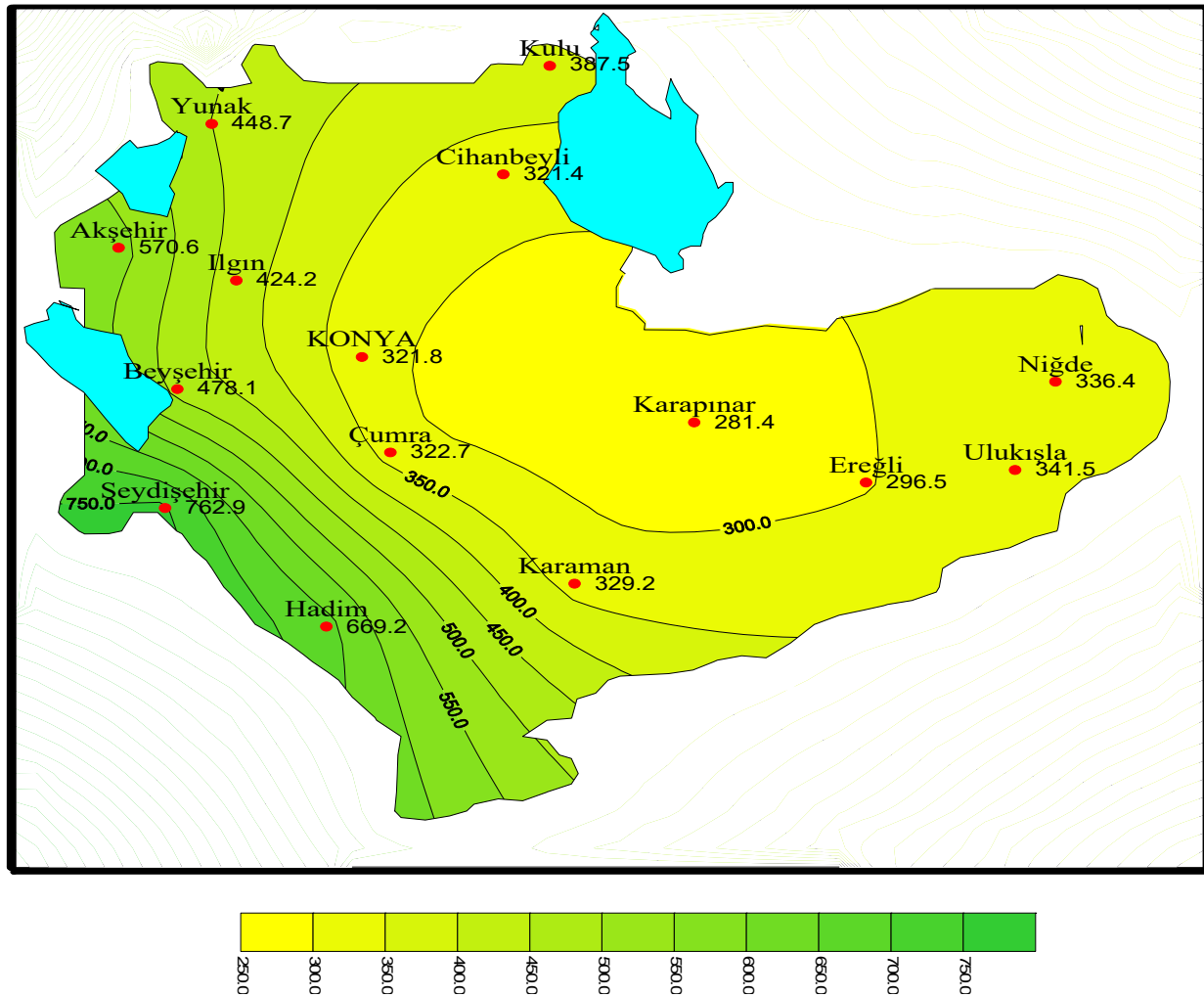
Fig. 1 Total annual precipitation of Konya region [7]
